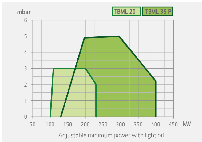
TBML 20
