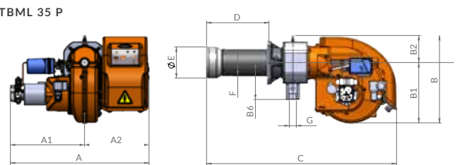
TBML 35 P
