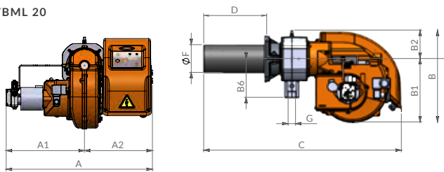
TBML 20
