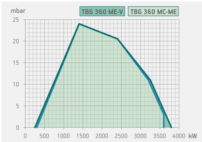
TBG 360 MC
