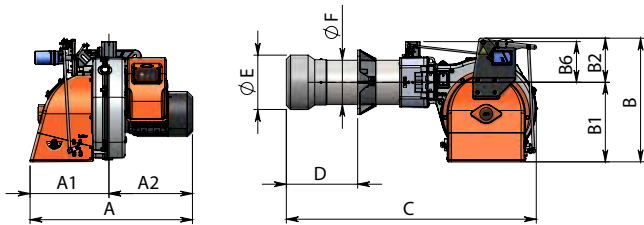
TBG 360 MC
