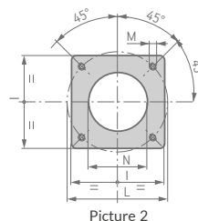
TBG 80-200 LX ME
